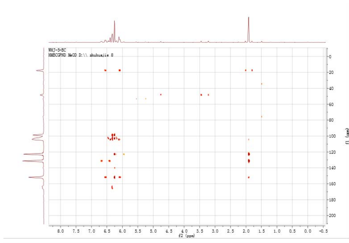
Fig.4 HMBC in CD 3 OD for compound 1
