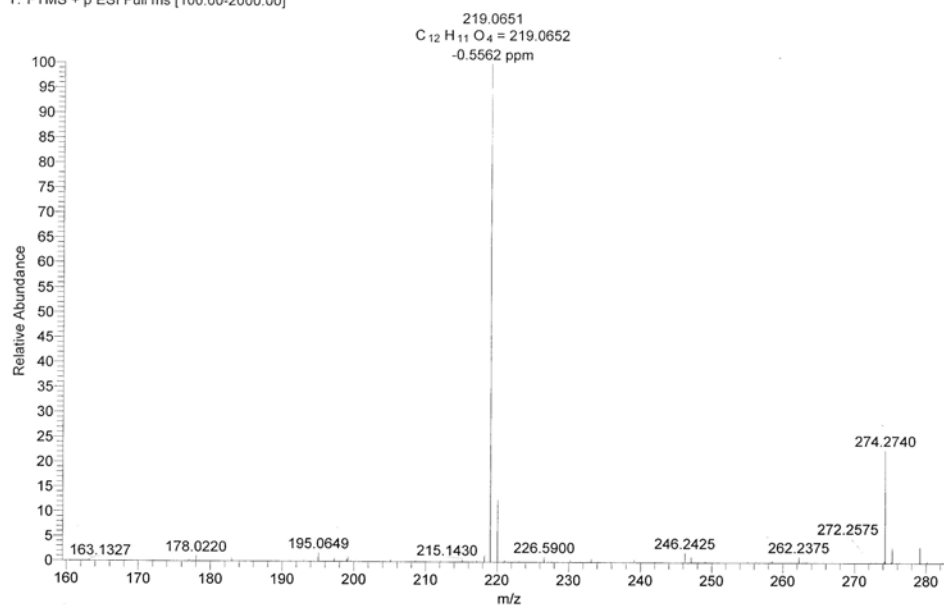
Fig.6 HRESIMS ( [M+H]^+ ) for compound 1
