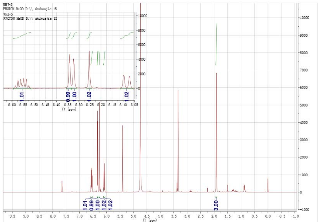
Fig.1 ^1\text{H} NMR in \text{CD}_3\text{OD} for compound 1
