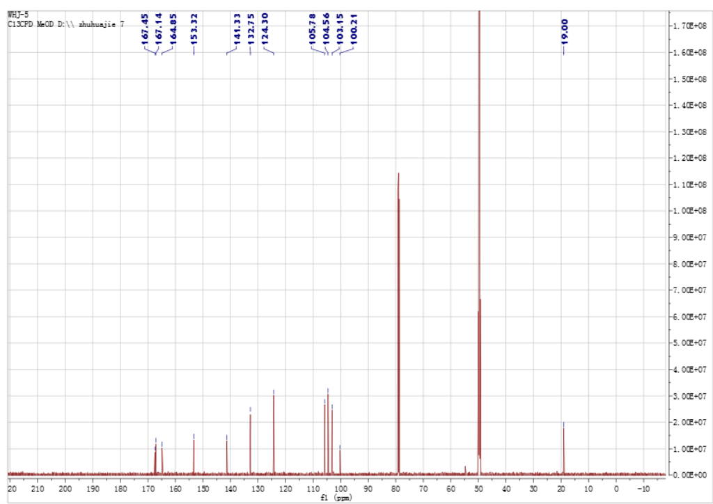
Fig.2 ^{13}\text{C} NMR in \text{CD}_3\text{OD} for compound 1
