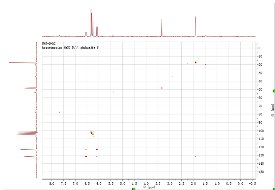
Fig.3 HSQC in CD 3 OD for compound 1
